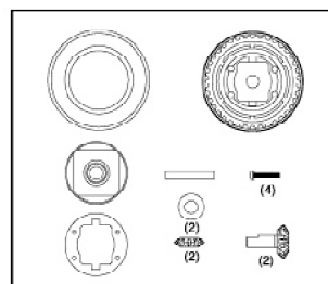
PD0801 DIFFERENTIAL SET
