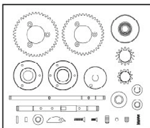
PD7675 2-SPEED, CLOSE RATIO TRANS
