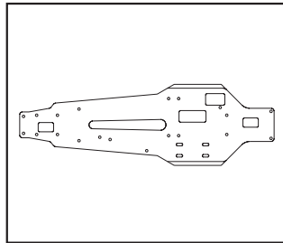
PD0834-L MAIN CHASSIS 2.5m/m
