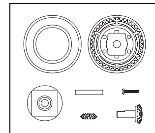
PD0801 DIFFERENTIAL SET
