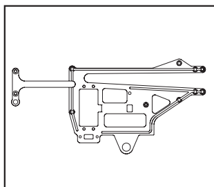
PD0957-S RADIO PLATE
