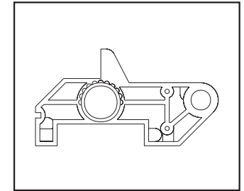
PD0831 RR BULKHEAD
